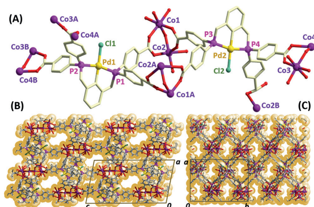
Figure 1. A) The asymmetric unit of the PCM-36 polymer framework showing Co II -carboxylate connectivity (pore constituents are omitted for clarity). [28] B) Space-filling and superimposed ball-and-stick representation in the crystallographic ac -plane showing the largest oval shaped pores. C) Alternative view in the ab -plane.
