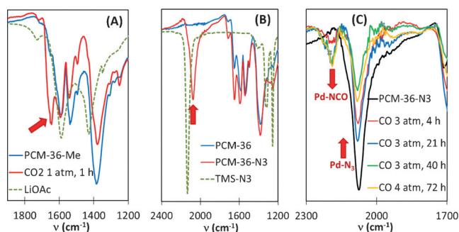
Figure 3. A) Comparison of solid-state FTIR spectra in the carbonyl stretching region as a function of PCM-36-Me exposure to CO 2 . B) The N 3 symmetric stretching band region. C) Appearance of NCO stretching band upon high pressure treatment of PCM-36-N 3 to CO.
