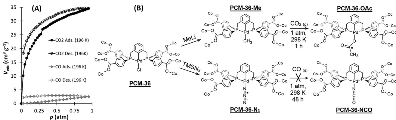
Figure 2. A) Adsorption-desorption isotherms for CO 2 and CO gas in PCM-36. B) Post-synthetic modifications applied to PCM-36 and reaction outcomes upon exposure of dry crystalline samples of modified PCM-36 to CO 2 and CO gas.
